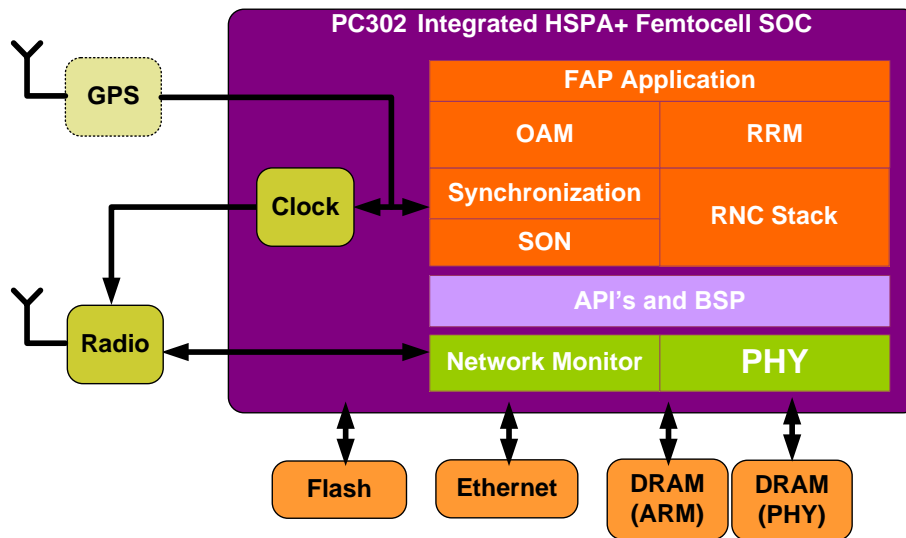
Figure 1 PC302 Femtocell System on Chip Architecture
