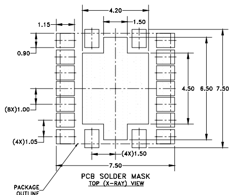
Figure 7: Recommended PCB Layout Information
