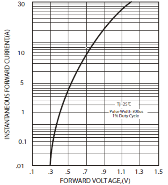
FIG.2-TYPICAL FORWARD CHARACTERISTICS
