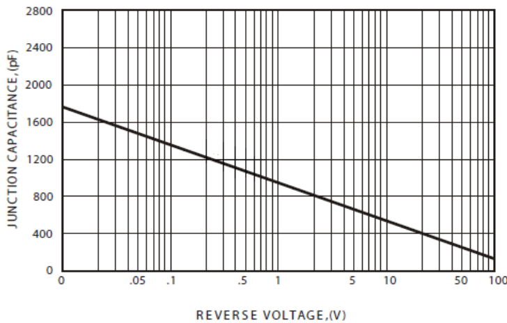
FIG.4-TYPICAL JUNCTION CAPACITANCE
